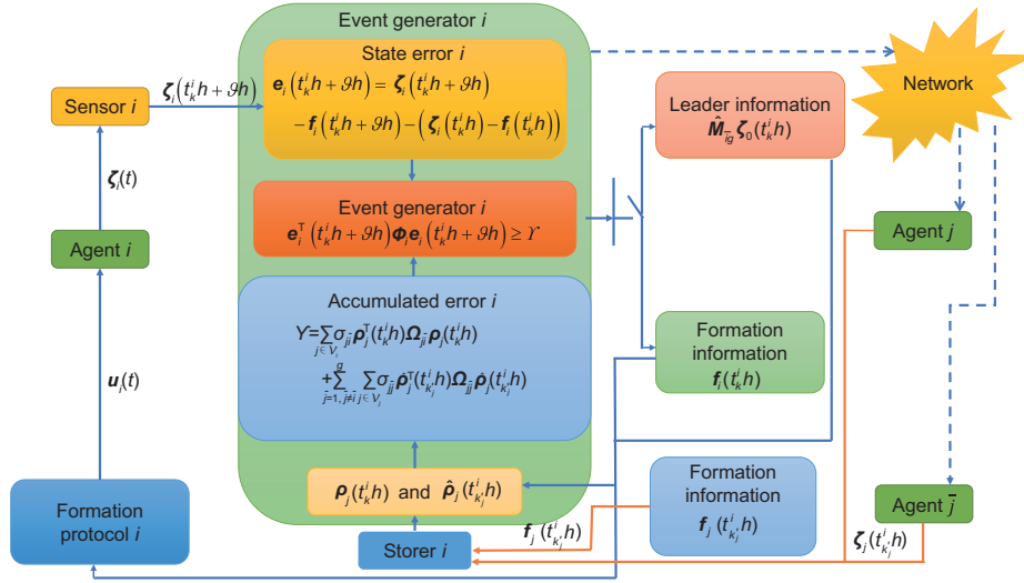
Fig. 2 Event-triggered distributed formation control for agent i
